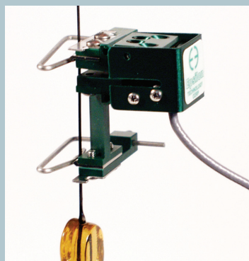
Model 3442 with 1 inch gauge length testing carbon fiber tow
