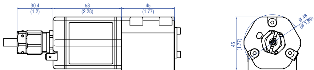
Fig. 3: Temposonics® RDV sensor electronics housing, part 2
