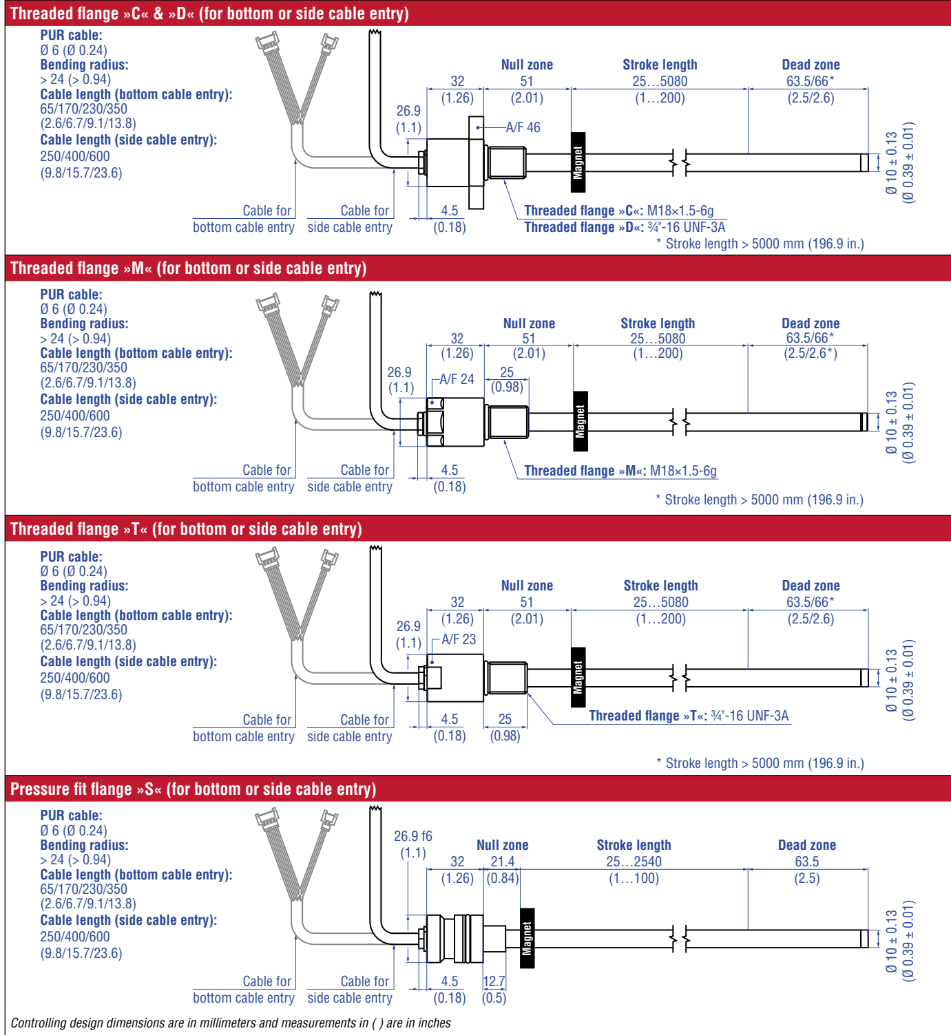
Fig. 3: Tempsonics® RDV flange types
