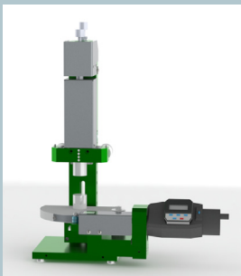
Model 3590-TORSION with a model 3590VHR axial calibrator
